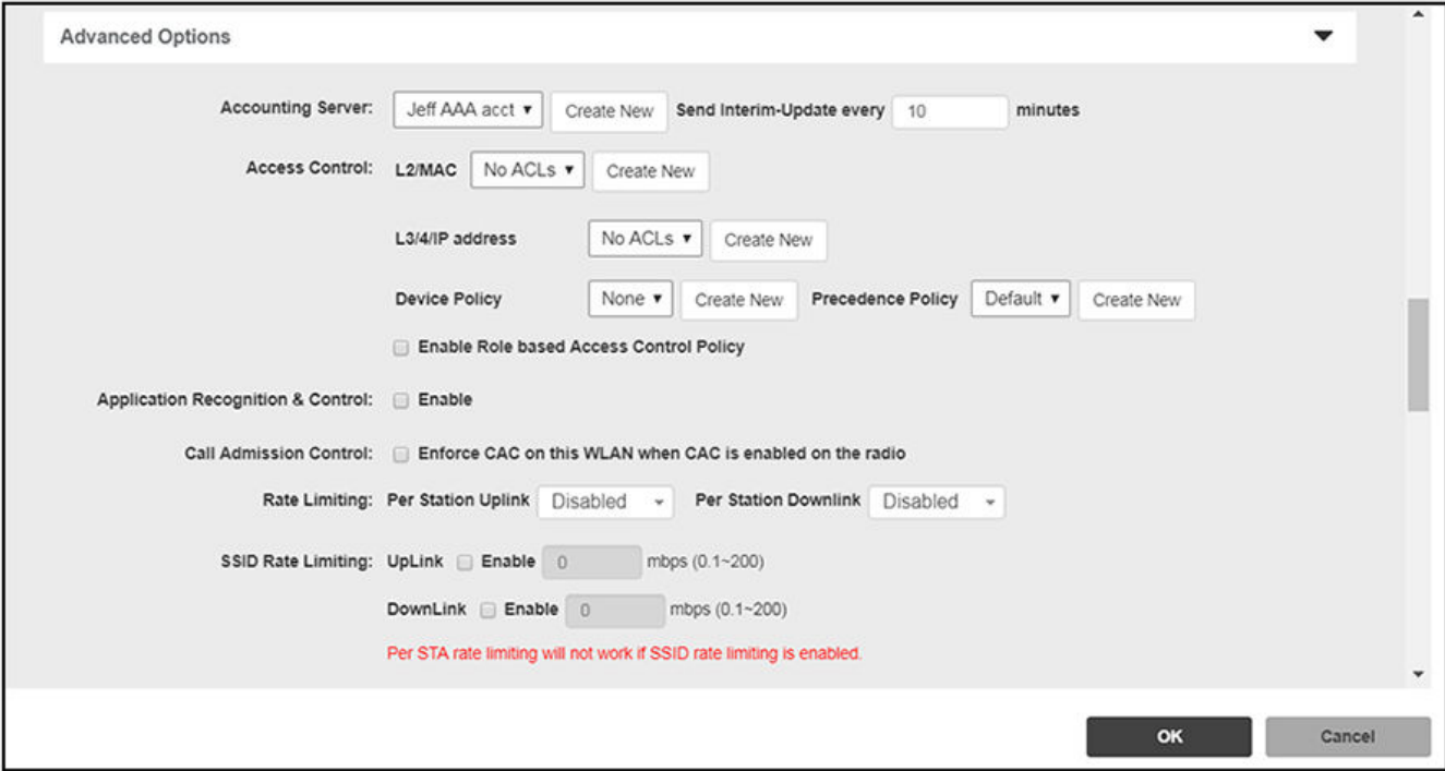
FIGURE 114 Select RADIUS Accounting Server on ZoneDirector
