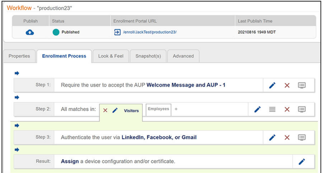
FIGURE 58 Publish Icon Under "Publish" Column
