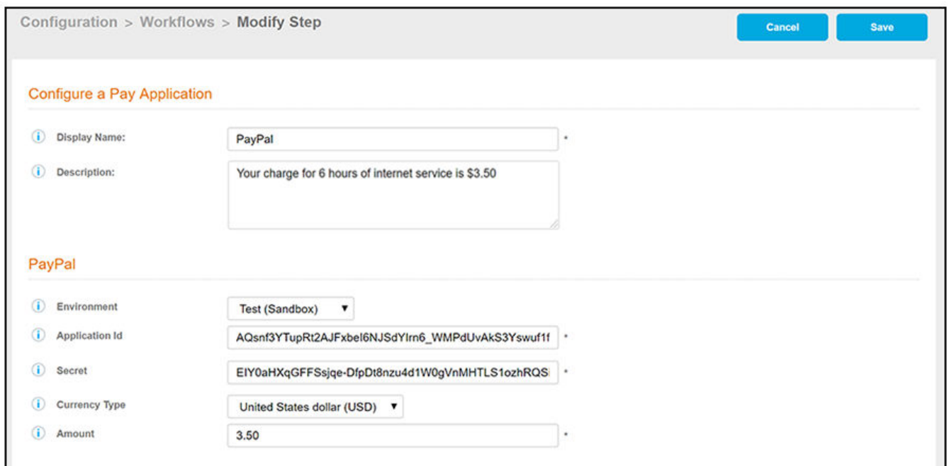
FIGURE 72 Cloudpath UI Pay Application Configuration Screen
